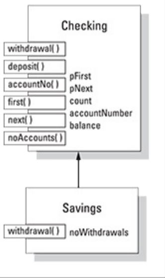
Figure 21-2: Savings implemented as a subclass of Checking.
