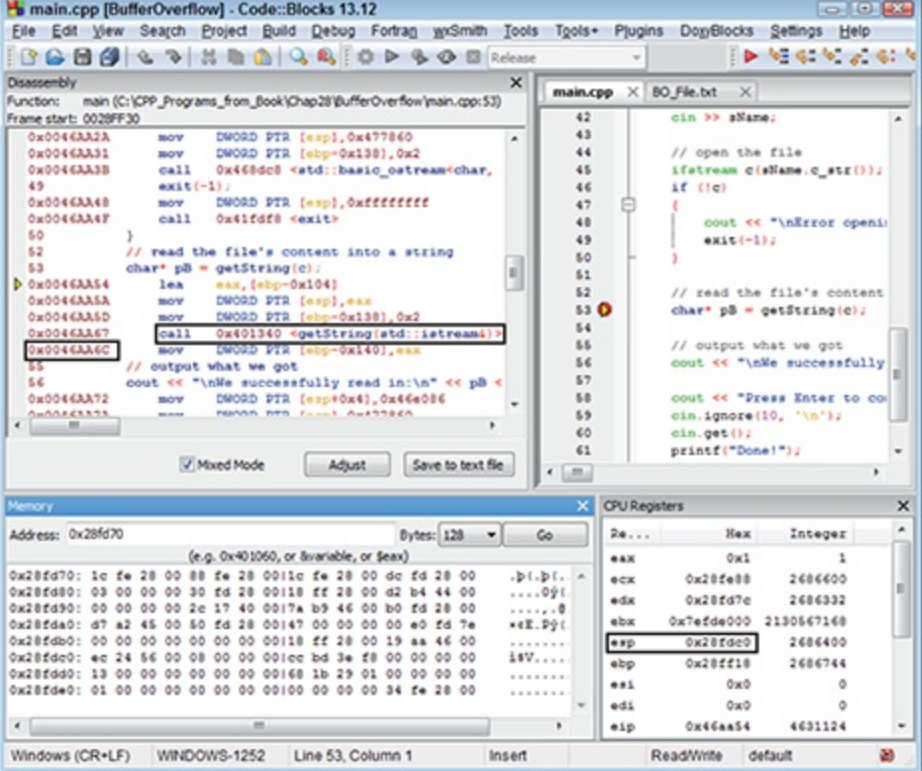
Figure 28-2: The ESP and the stack memory immediately before the call to getString() .
