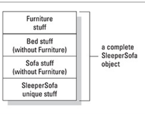
Figure 25-5: Memory layout of SleeperSofa with virtual inheritance.
