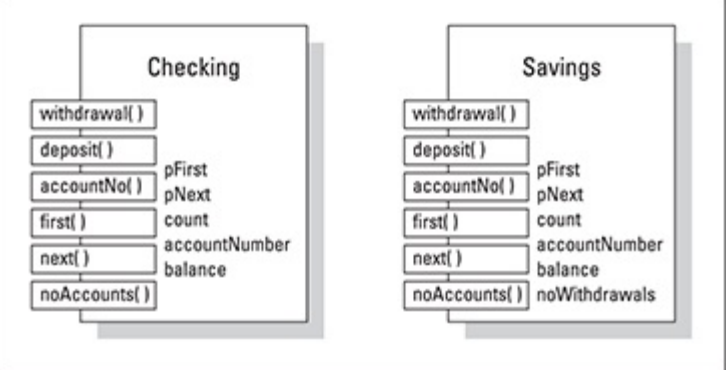
Figure 21-1: Independent classes Checking and Savings .
